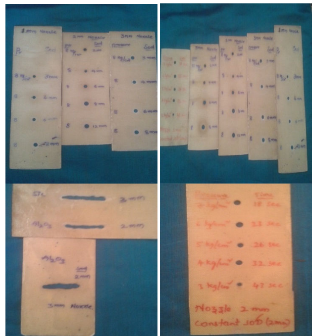
Fig. 5 Results obtained on FRP composites at various pressures, SOD's, and Nozzle diameters
