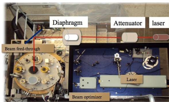
Fig. 6 Experimental setup of the laser beam
