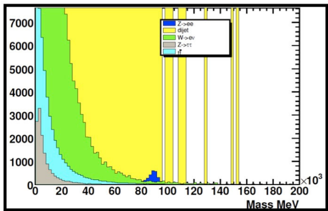
Fig. 7 The reconstruction of the invariant mass of the Z to e^+e^- signal to background
