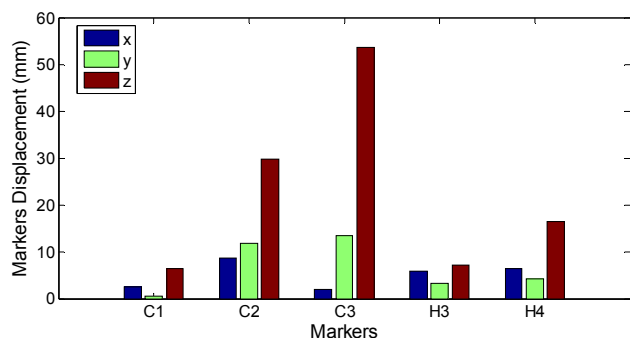
Fig. 11 Markers displacements (magnitude), extension
