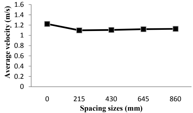
Fig. 17 The changes in average velocities when spacing sizes were increased for rhombus array arrangement
