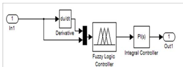
Fig. 6 Implementation of Fuzzy Logic Controller in MATLAB
