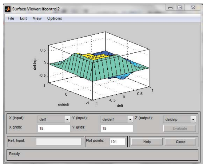
Fig. 5 (b) Output Surface Viewer in MATLAB
