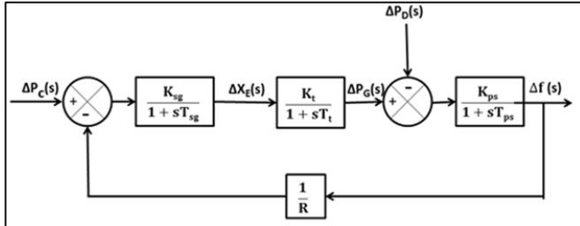
Fig. 1 Single Area Control Model
