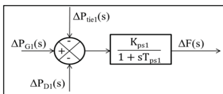
Fig. 2 Change in frequency for Two Area control
