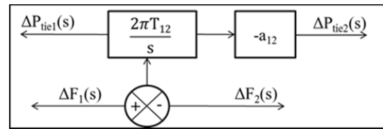
Fig. 3 Tie line power in Area-2
