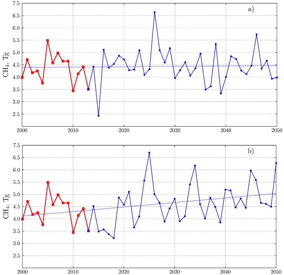
Figure 5. Annual methane emission from wetland complexes of Western Siberia obtained using the RegCM4/CLM4.5 data. The initial and lateral boundary conditions for the period 2000–2013 (bold red line) are provided by the NCEP-DOE AMIP-II (R2) (Kanamitsu et al. 2002) reanalysis and for the period 2013–2050 (bold blue line) according to the global model HadGEM2-ES (Collins et al. 2011) for RCP 4.5 (a) and RCP 8.5 (b) scenarios. Dashed blue lines are the growth rate of methane emission.
