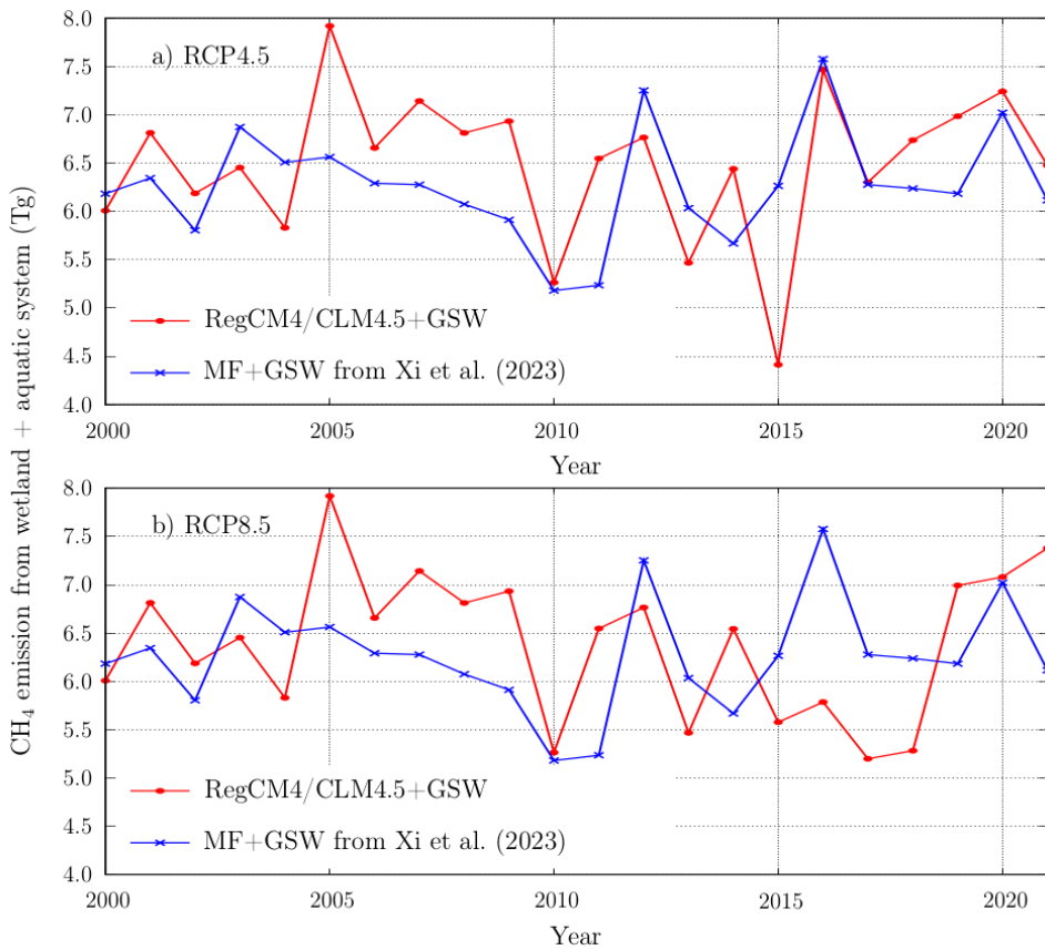
Figure 6. Total methane emission from wetland and aquatic system of the Western Siberia region from 2000 to 2021 for RCP 4.5 (a) and RCP 8.5 (b) scenarios. Blue points and line are results of Xi et al. (2023), red points and line are our results obtained within RegCM4/CLM4.5 model for 2000–2021.
