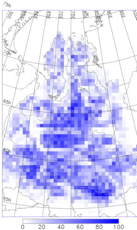
Figure 2. Wetland complexes of Western Siberia and their fractions on a 40×40 km grid of the RegCM4 model according to data from (Sheng et al. 2004).
