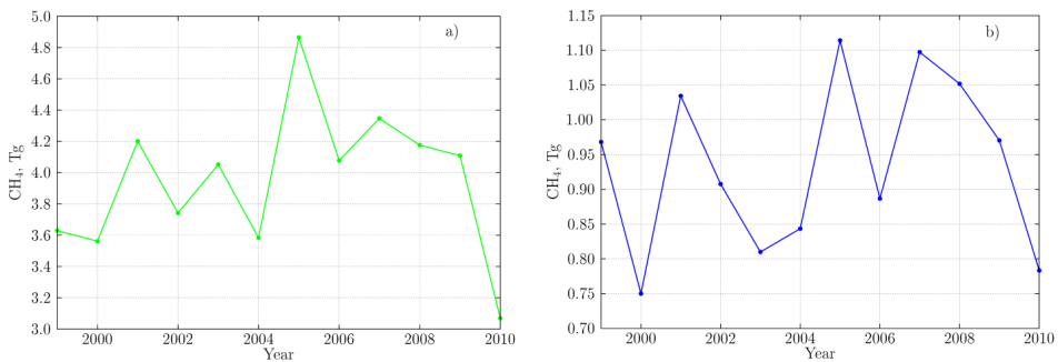
Figure 4. Methane emissions from the wetland complexes in Western Siberia in 1999–2010 according to the results of the RegCM4/CLM4.5 model: a) taiga zone; b) the territory of the Tomsk region.
