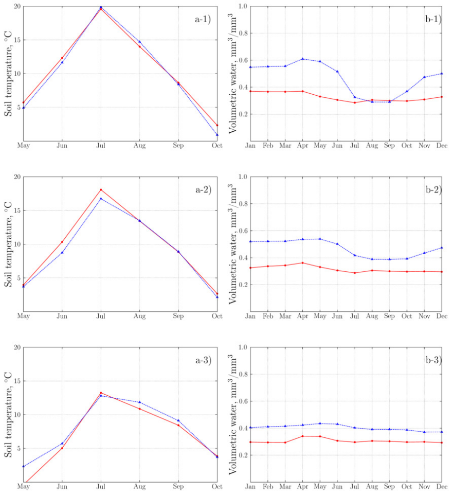
Figure 3. Comparisons of ERA5 reanalysis (Hersbach et al. 2020) (solid red line) and RegCM4/CLM4.5 data (dashed blue line) for soil temperature (a) and volumetric moisture content (b) for the study domain in three ERA5 soil layers: (1) – layer 0–7 cm, (2) – layer 7–49 cm, (3) – layer 49–91 cm.
