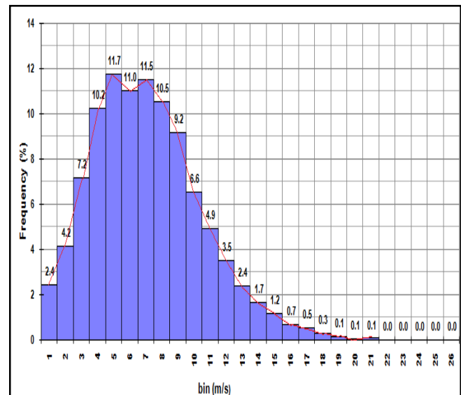
Fig. 3 Wind Speed Distribution 20m
