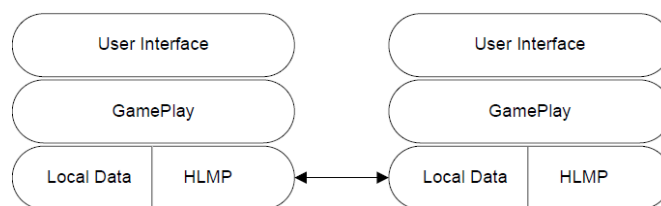
Fig. 1 Magic Race basic architecture
