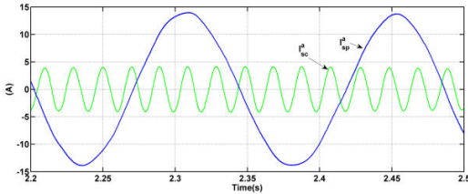
Fig. 23 (b) Zoom of Stator currents of PW and CW ( i_{sc}^a, i_{sp}^a )
