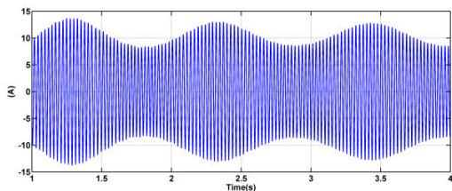
Fig. 24 Rotor current ( i_r^d )
