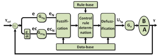
Fig. 7 Block diagram of PD-like Fuzzy Logic Controller
