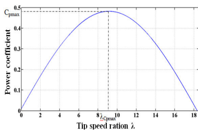
Fig. 2 Power coefficient for the wind turbine model
