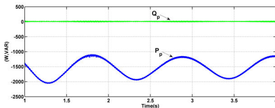
Fig. 25 Stator active and reactive powers ( P_p, Q_p )
