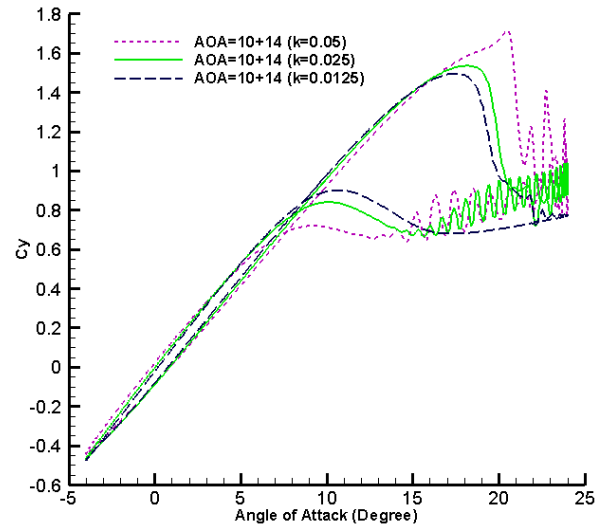
Fig. 2 Effect of reduced frequency on hysteresis loop
