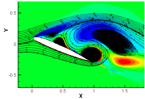
Fig. 8 Vorticity contour superimposed with streamlines of CFD at 23° upstroke
