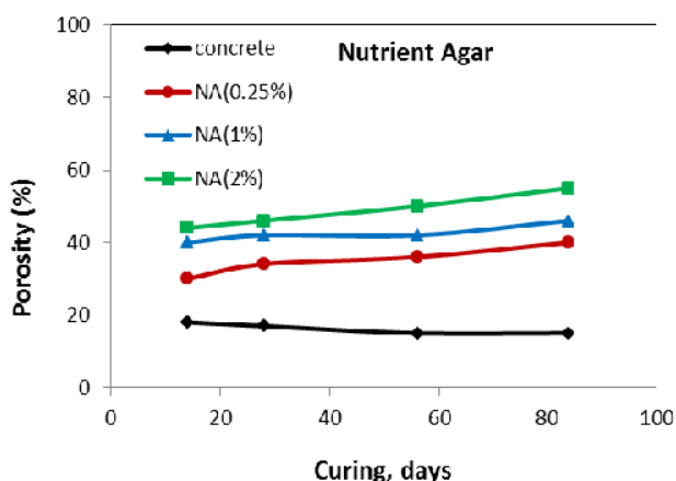
Fig. 2 Porosity increase of specimens during concrete curing
