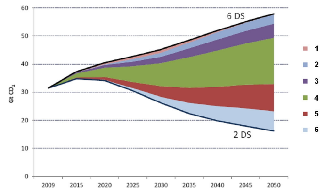
Fig. 2 Efficiency improvements and fuel switching in the end-use sectors account for more than half of the reductions [15]
