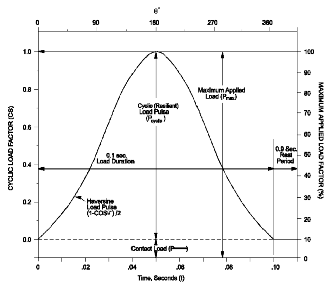
Fig. 4 The loading cycle waveform ([20])
