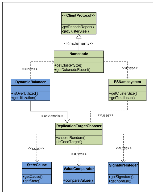
Fig. 3 Class diagram for some of additional features to existing Hadoop block placement policy
