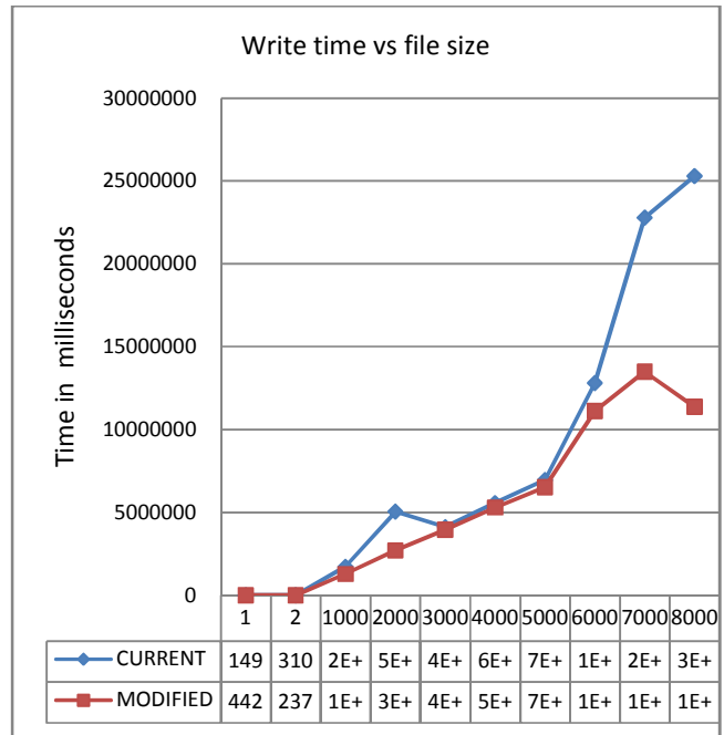
Fig. 11 Write time comparisons between new and original replication target chooser logic in HDFS system
