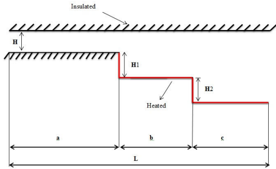
Fig. 1 Geometry domain
