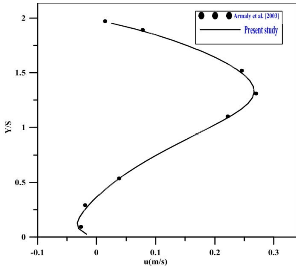
Fig. 2 (b) Profile of velocity at X/S=3
