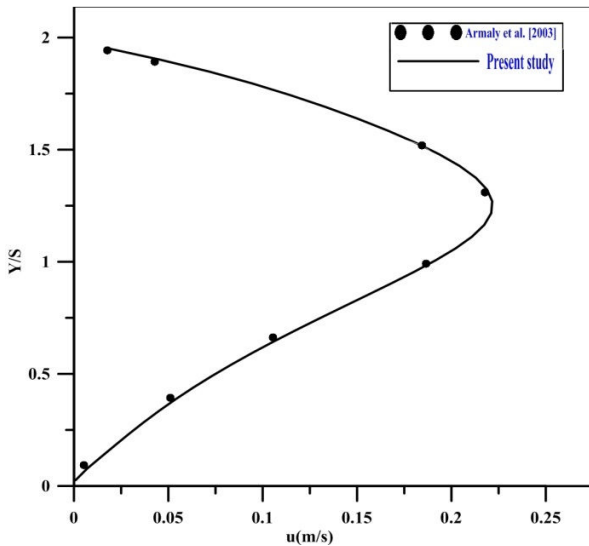
Fig. 2 (c) Profile of velocity at X/S=5
