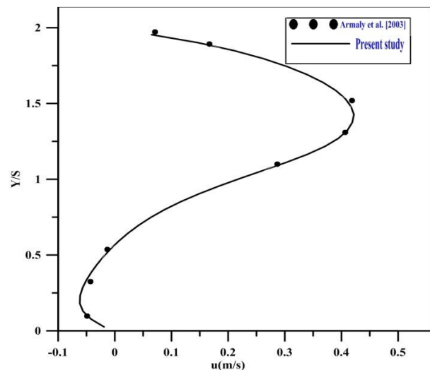
Fig. 2 (a) Profile of velocity at X/S=1
