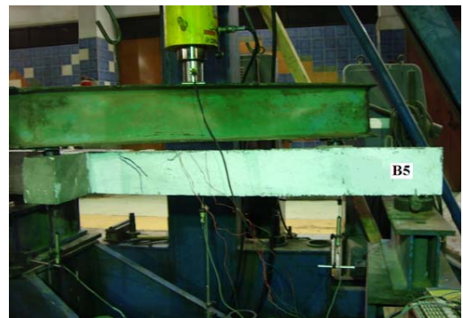
Fig. 4 (f) Failure modes and crack patterns of the tested beam B5
