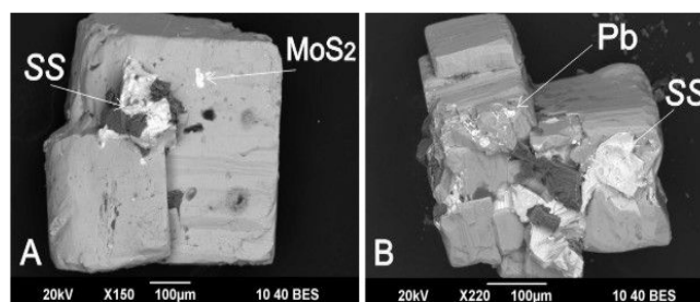
Fig. 3 Growths of Zn-containing grey copper ore (SS), inclusions of molybdenite (A) and native lead+anglesite? phases (B) on surfaces of pyrite grains, Gumeskhi
