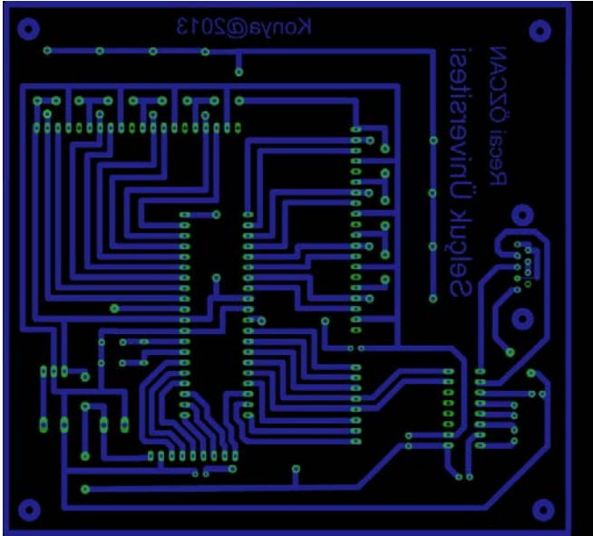
Fig. 1 PCB of designed system
