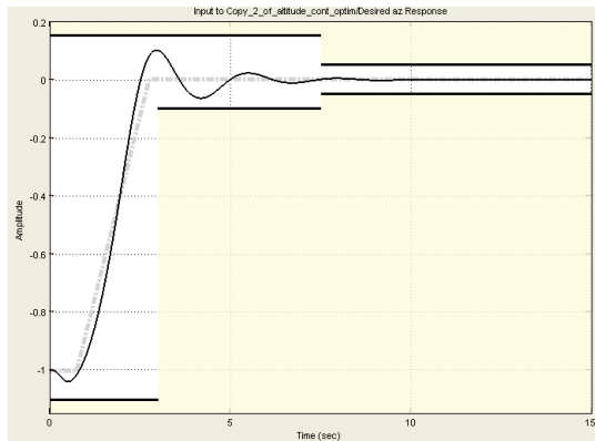
Fig. 4 Pre-Optimization Response
