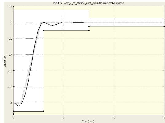
Fig. 5 Optimized Solution
