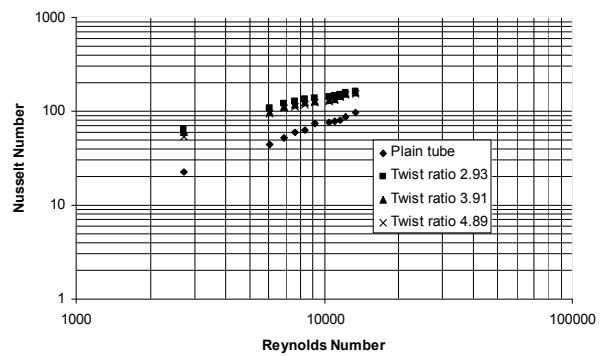
Fig. 5 Nusselt number vs Reynolds number of kenics insert 300 R and 300 L with 100 spacer under turbulent flow
