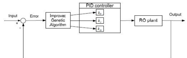
Fig. 3 Schematic of auto tuning PID controller based on improved GA function [1]
