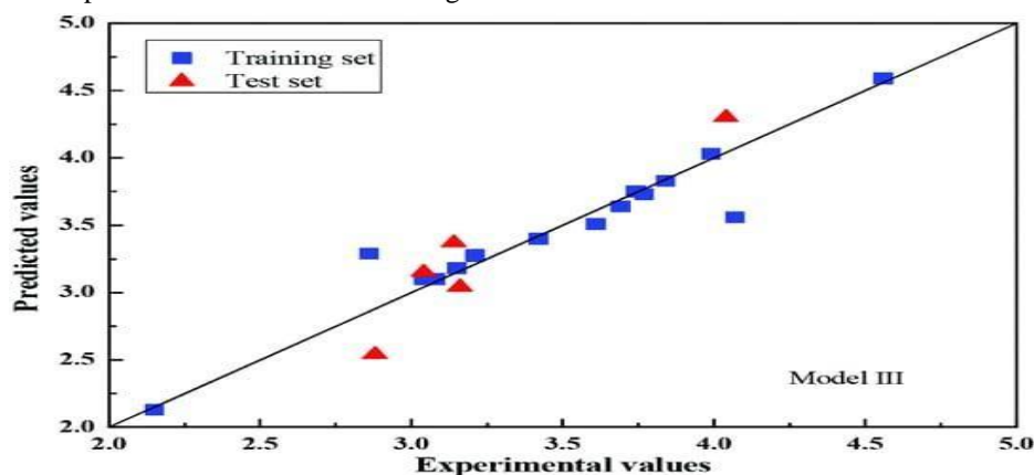
Fig.3. Plot of predicted vs experimental log 10 (LC 50 ) values for model III.
