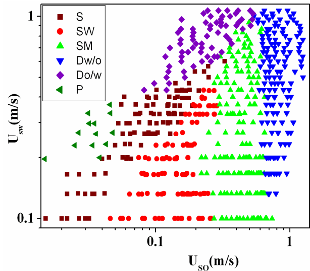
Fig. 5 Experimental flow pattern map (◀- plug flow (P), ■- slug flow (S), ●-wavy stratified flow (SW), ▲- Stratified mixed flow (SM), ▼-water dispersion in oil flow ( D_{w/o} ), ◆ - oil dispersion in water flow( D_{o/w} ))
