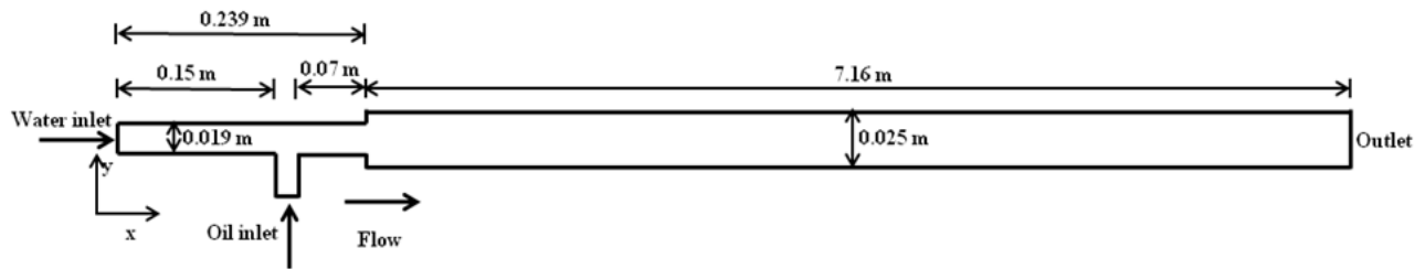
Fig. 1 Schematic of model geometry
