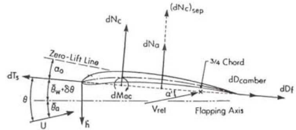
Fig. 4. Wing section aerodynamic forces and motion variables
