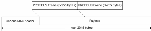
Fig. 8 Encapsulation of a PROFIBUS frame into an IEEE 802.16 MAC PDU
