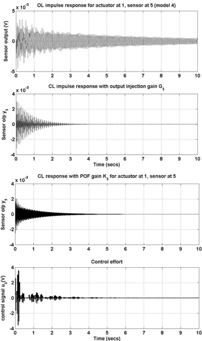
Fig. 10 OL / CL response with G and K / control u for model 4
