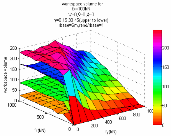
Fig. 21 Variation of f_y and f_z on the workspace volume for (r_{\text{end}}/r_{\text{base}})=1
