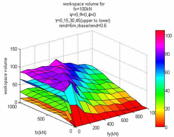
Fig. 23 Variation of f_y and f_z on the workspace volume for (r_{\text{base}}/r_{\text{end}})=0.6
