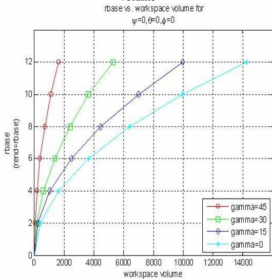
Fig. 14 The effect of the size of BP on the basis of workspace volume
