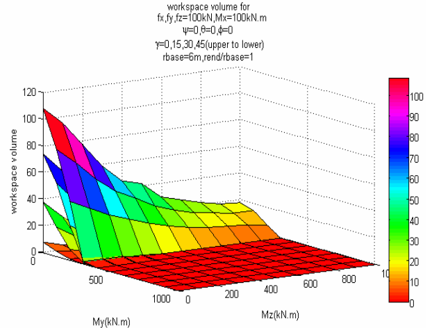
Fig. 27 Variation of M_y and M_z on the workspace volume for (r_{\text{end}}/r_{\text{base}})=1
