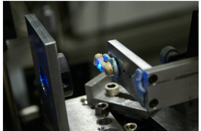
Fig. 12 One of the ceramic fixed partial denture sample in front of the scanning head of the OCT
