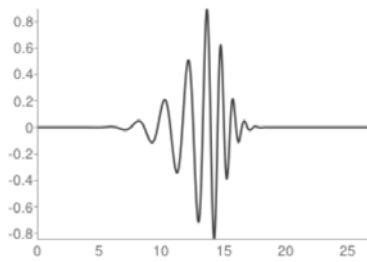
Fig. 7. Daubechies Wavelets 'db14'
