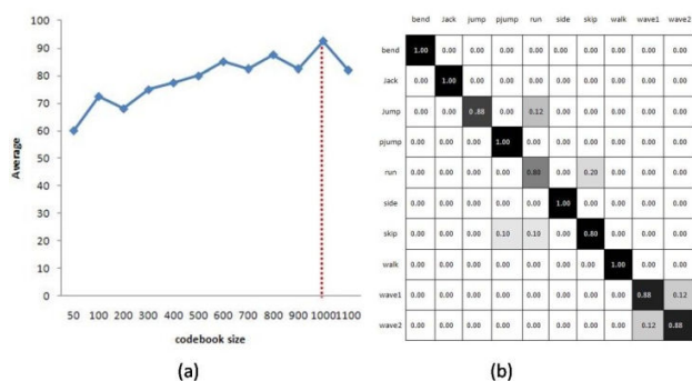
Fig 10 Results for the Wierzman dataset (a) shows the average accuracy as a function of codebook size, (b), shows results for an SVM classifier
