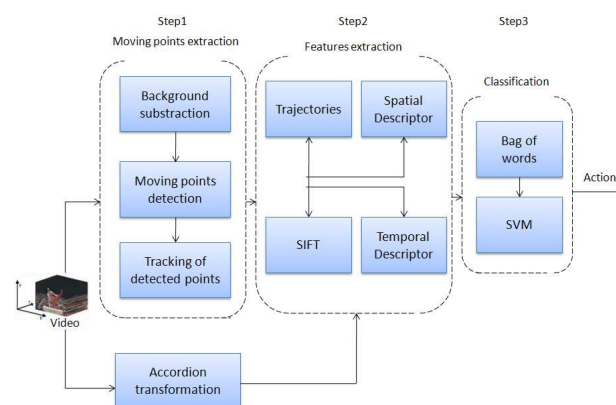
Fig. 1 Overview of our proposed framework
