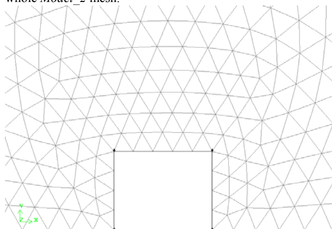
Fig. 7 Main geometrical features of Model_0 grid refinement near the model building
