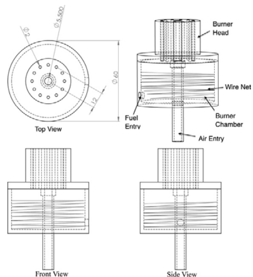
Fig. 1 IDF Burner Construction
