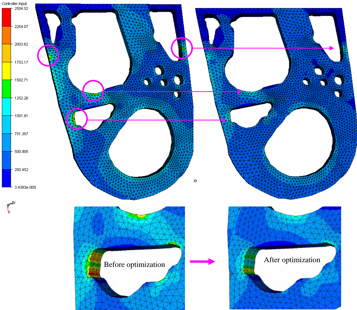
Fig. 10 Shape optimization
