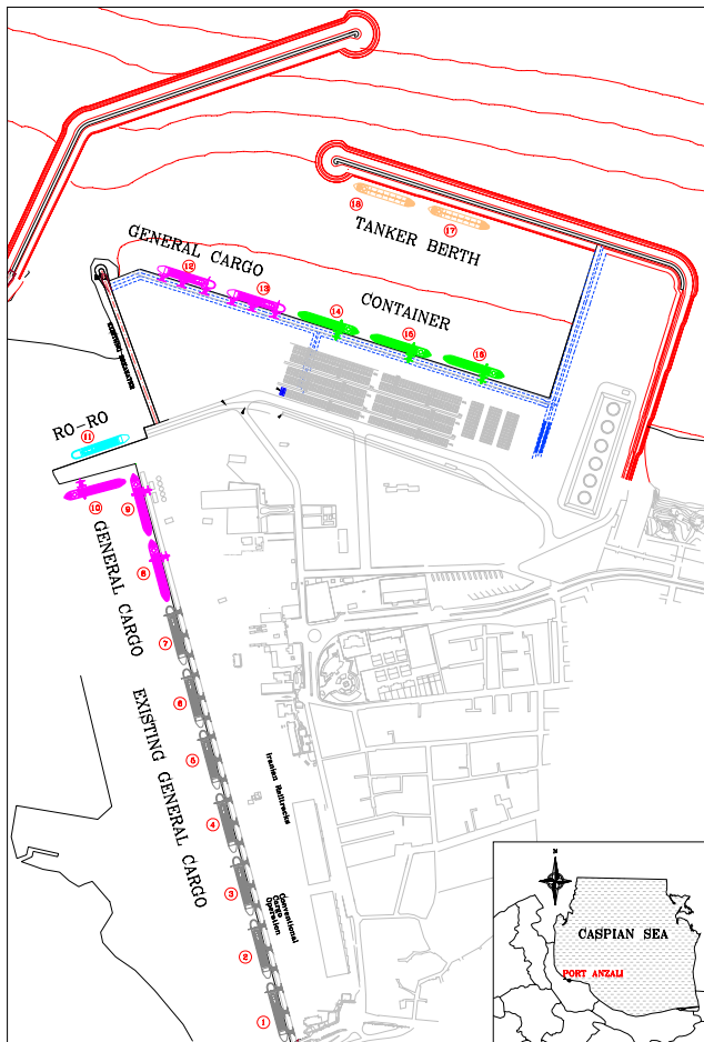
Fig.3. Proposed port layout for 2016
