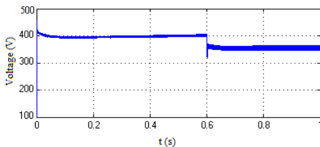
Fig. 12 Battery terminal voltage
