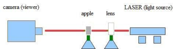
Fig. 1 Experimental setup adopted for the optical test
