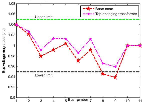
Fig.6 Comparison of bus voltage magnitude (Tap Changing Transformer)
