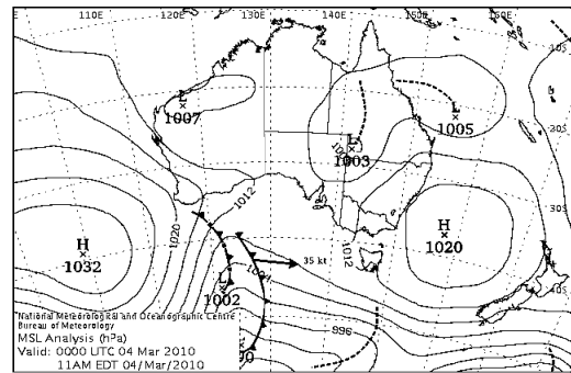
Fig. 5 Top: Wind induced currents during a period of non-cyclic sea breeze patterns Bottom: Synoptic map of Australia depicting an incoming high pressure system, the low trough east of the WA coast
