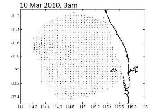
Fig. 7 Top: Wind induced currents during a period of non-cyclic sea breeze patterns Bottom: Synoptic map of Australia depicting a passing high, the low trough east of the WA coast
