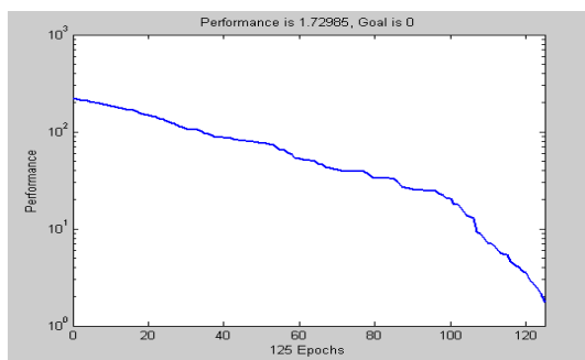
Fig. 5 Performance result of RBF model, Neurons = 125, MSE = 1.72985
