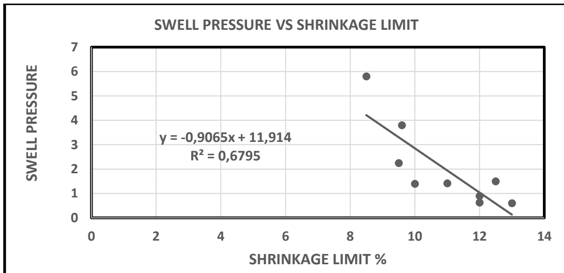
Drawing 1: Swelling pressure versus shrinkage limit, for location 1.
