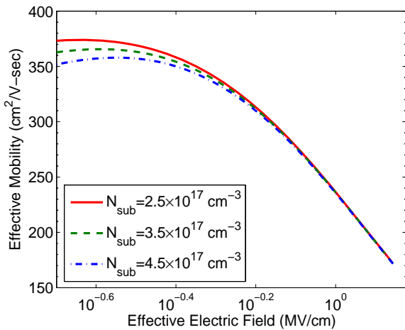
Fig. 12. Effective mobility vs. effective electric field for different substrate concentrations ( N_{sub} ) with L = 0.1 \mu\text{m} , N_{pm} = 1.75 \times 10^{18} \text{ cm}^{-3} , L_p = 25 nm, V_{DS} = 0.05 V, T = 300 K
