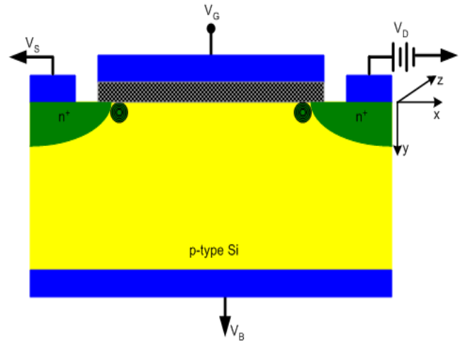
Fig. 6. Pocket implanted n-MOSFET structure
