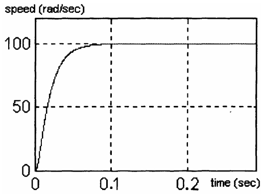
Fig. 3a Speed response
