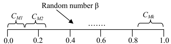
Fig. 2 Morphactin concentration state space
