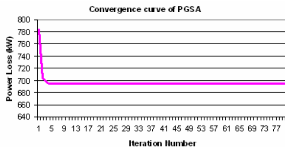
Fig. 5 Convergence curve of PGSA
