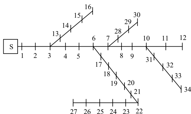
Fig. 6 34 - bus distribution network configuration
