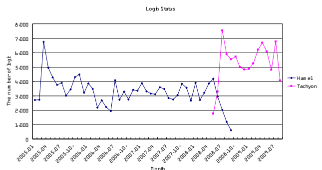
Fig. 1. Login Statistics
