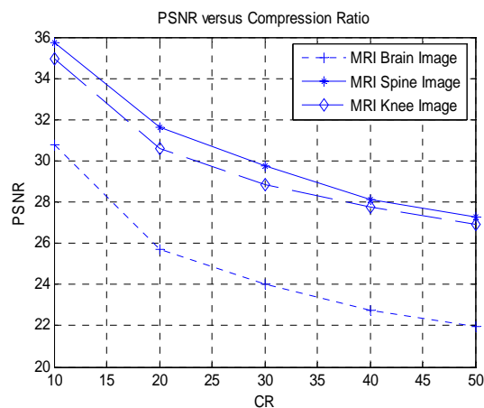
Fig. 4 PSNR and Compression ratio of MRI test images
