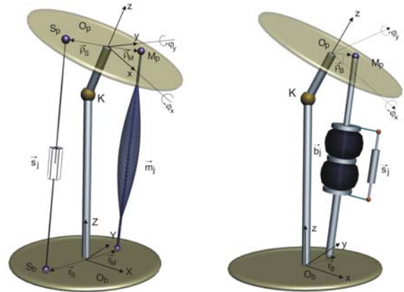
Fig. 1 PMA and PBA module structures
