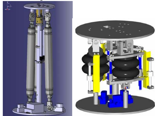
Fig. 2 Modules design
