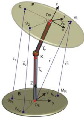
Fig. 3 Modules model
