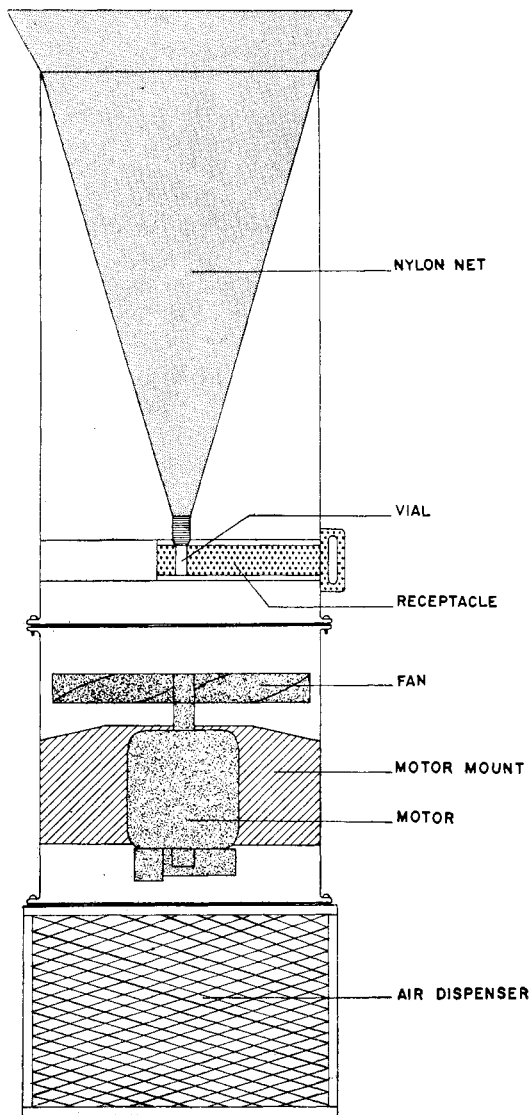
Fig. 1. Suction trap.
