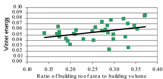
Fig. 8 Winter energy (kWh/m 2 /day) of the sample schools
