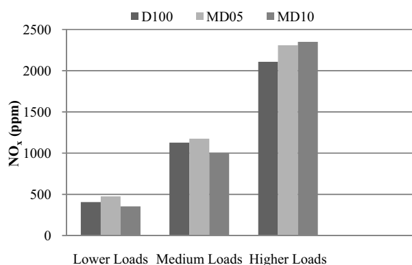
Fig. 11 Emission of NO x at various loads
