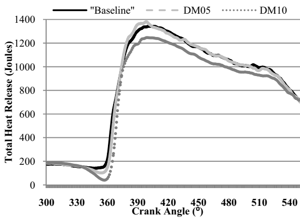
Fig. 5 Cumulative heat release for test fuels
