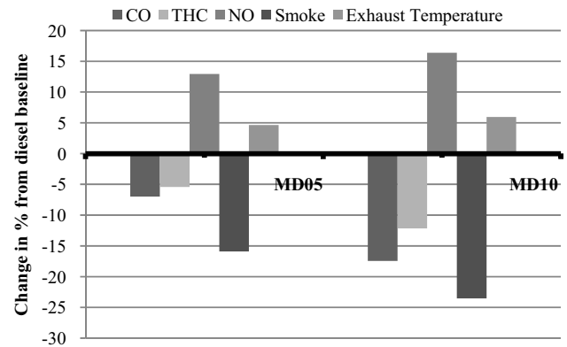
Fig. 13 Percentage change in full load emission of CO, THC, Smoke and Exhaust Temperature compared to diesel baseline
