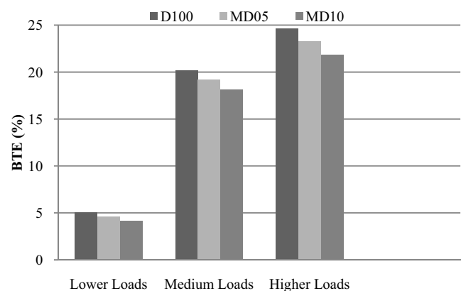
Fig. 14 BTE for test fuels at various loads
