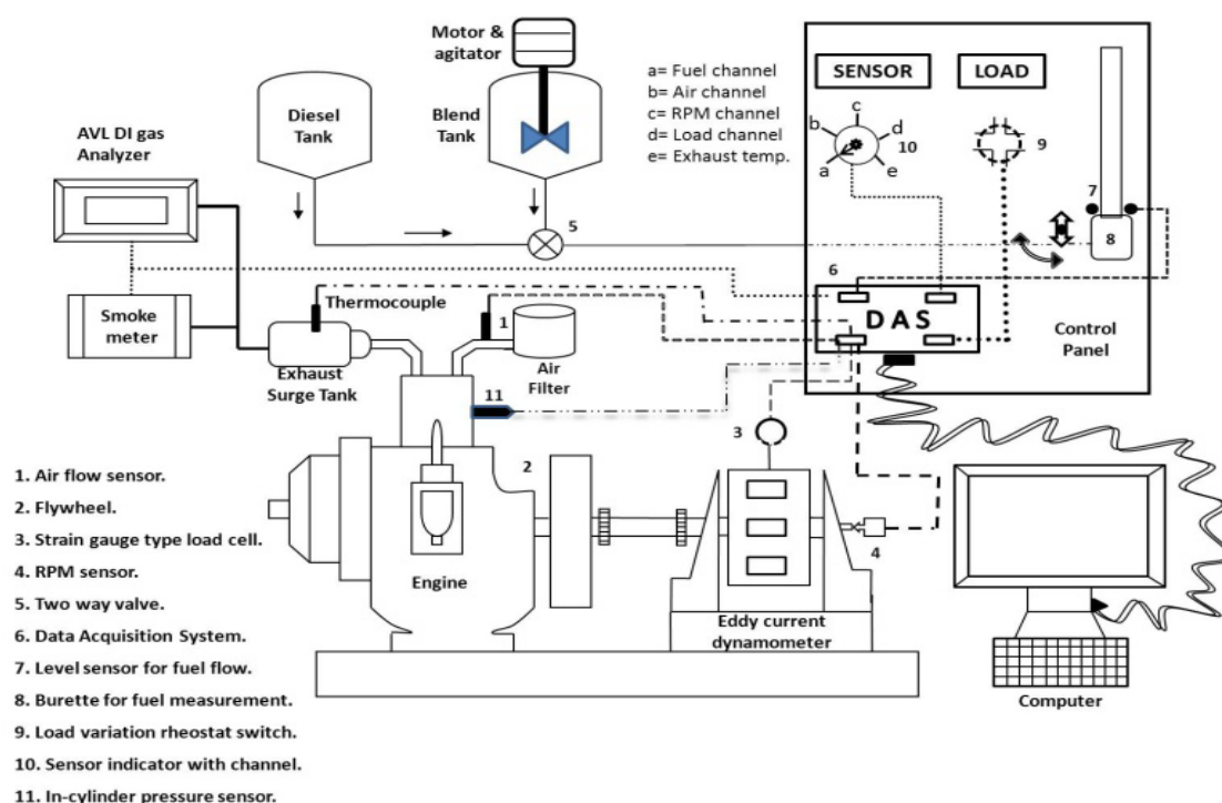
Fig. 1 Engine test rig lay out
