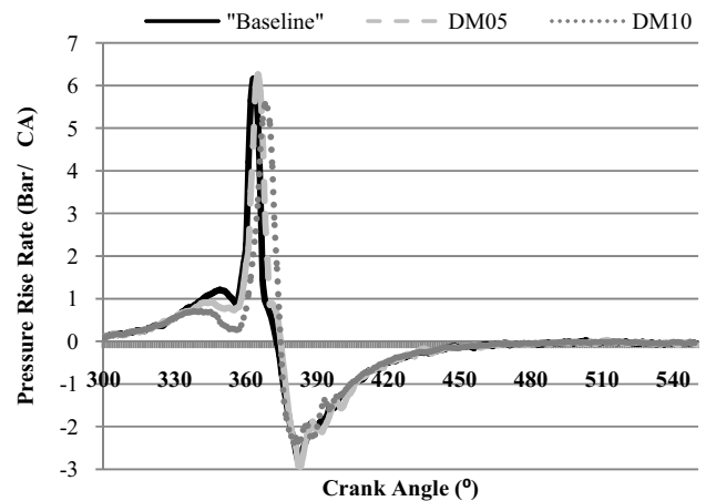
Fig. 3 Pressure rise rate diagram for test fuels
