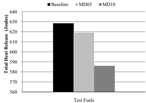
Fig. 8 Total cyclic heat release in Joules
