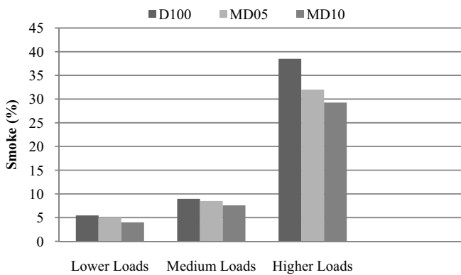
Fig. 12 Smoke opacity at various loads
