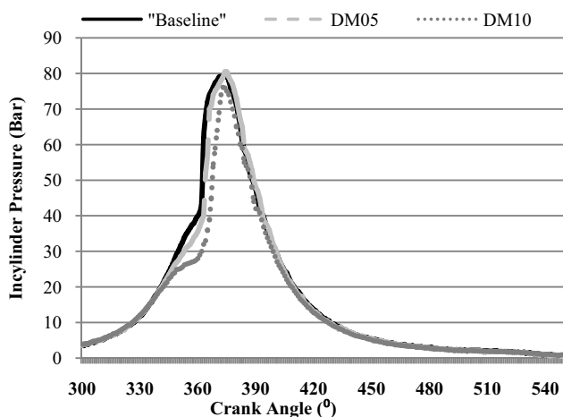
Fig. 2 Pressure-crank angle diagram for test fuels
