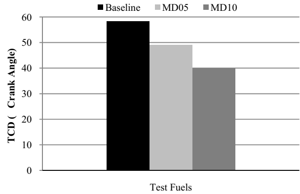
Fig. 7 Total combustion duration in °CA
