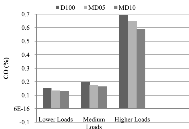
Fig. 9 Emission of CO at various loads
