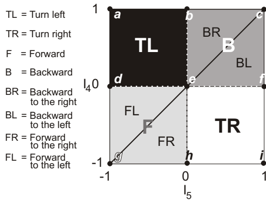
Fig. 6. Plot of the input space ( I_4, I_5 , see Fig. 5) which is classified into four main areas. For input values in a dark square area ( dabe ), the walking machine will perform spot turning to the left with different radians while a white square area ( efih ) is for the right turn. In light gray triangle areas ( gde and geh ), they will move forward in different curves to the left and the right and dark gray triangle areas ( ebc and ecf ) are for backward to the right and the left, respectively. Additionally, if I_4 and I_5 are varied along the diagonal line ( gac ), the machines will walk straight forward ( ge ) and backward ( ec ) with different walking speeds. Details on robot walking experiments have been presented in [9]
